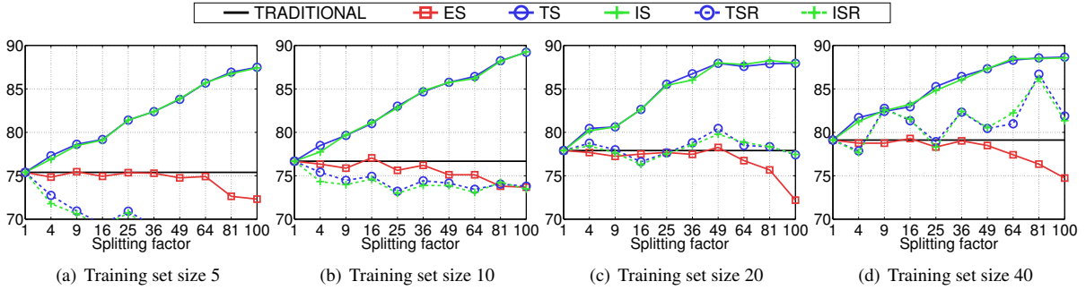
Fig. 3. Classification accuracies (vertical axis): LBP with local splitting.
