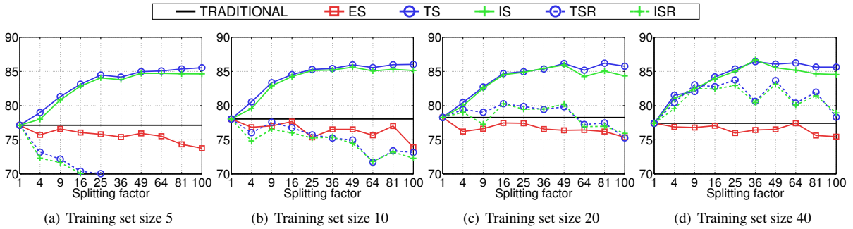
Fig. 4. Classification accuracies (vertical axis): LTP with local splitting.
