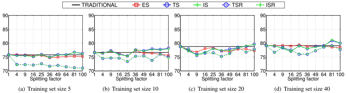
Fig. 5. Classification accuracies (vertical axis): LBP with periodic splitting.
