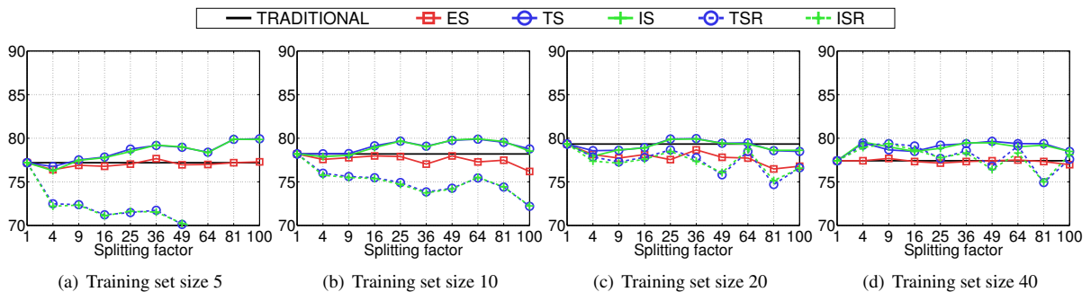
Fig. 6. Classification accuracies (vertical axis): LTP with periodic splitting.
