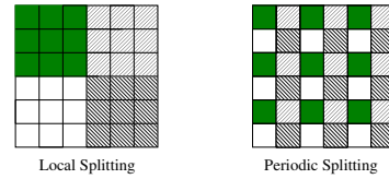
Fig. 2. Schema of the two splitting strategies (for n = 4 ). Similarly colored patterns are collected into one histogram.
