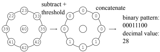
Fig. 1. Schematized flow of LBP computation.
